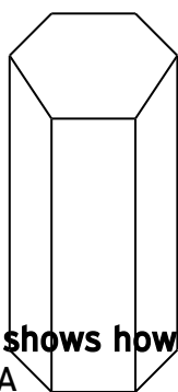
Monoclinic sulphur
